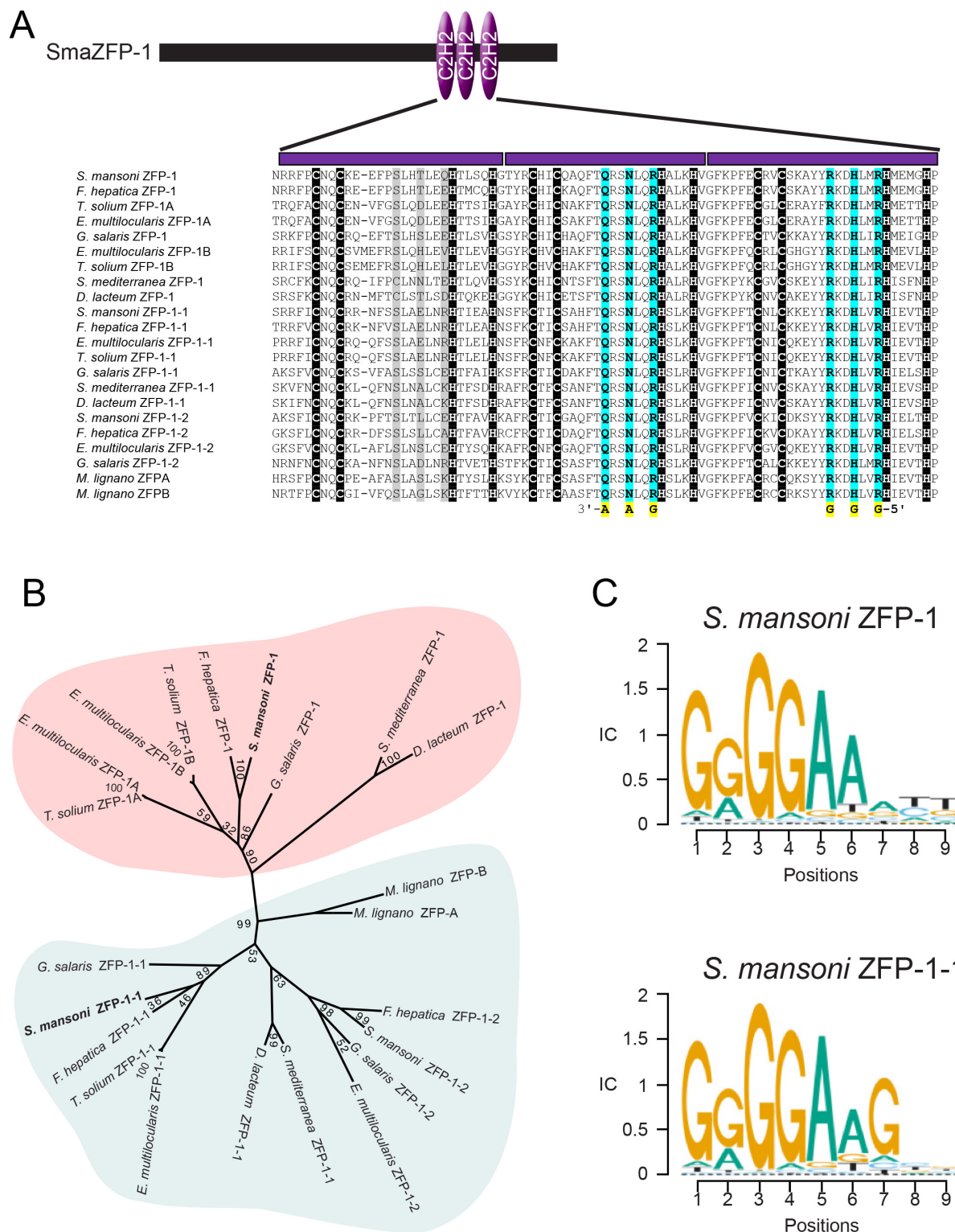
Figure 4. ZFP-1 and ZFP-1-1 are flatworm specific zinc finger proteins and are putative transcriptional regulators. (A) Multiple protein sequence alignment of the C2H2 domain of several zfp-1 and zfp-1-1 homologs. Zinc coordinating residues are shown in black background. Conserved residues contributing to high specificity DNA-binding are highlighted in cyan for the second and third zinc fingers, with the specific DNA base shown below the residue highlighted in yellow. The corresponding positions in the first zinc finger are shown in grey background. The positions determining DNA Figure 4 continued on next page
