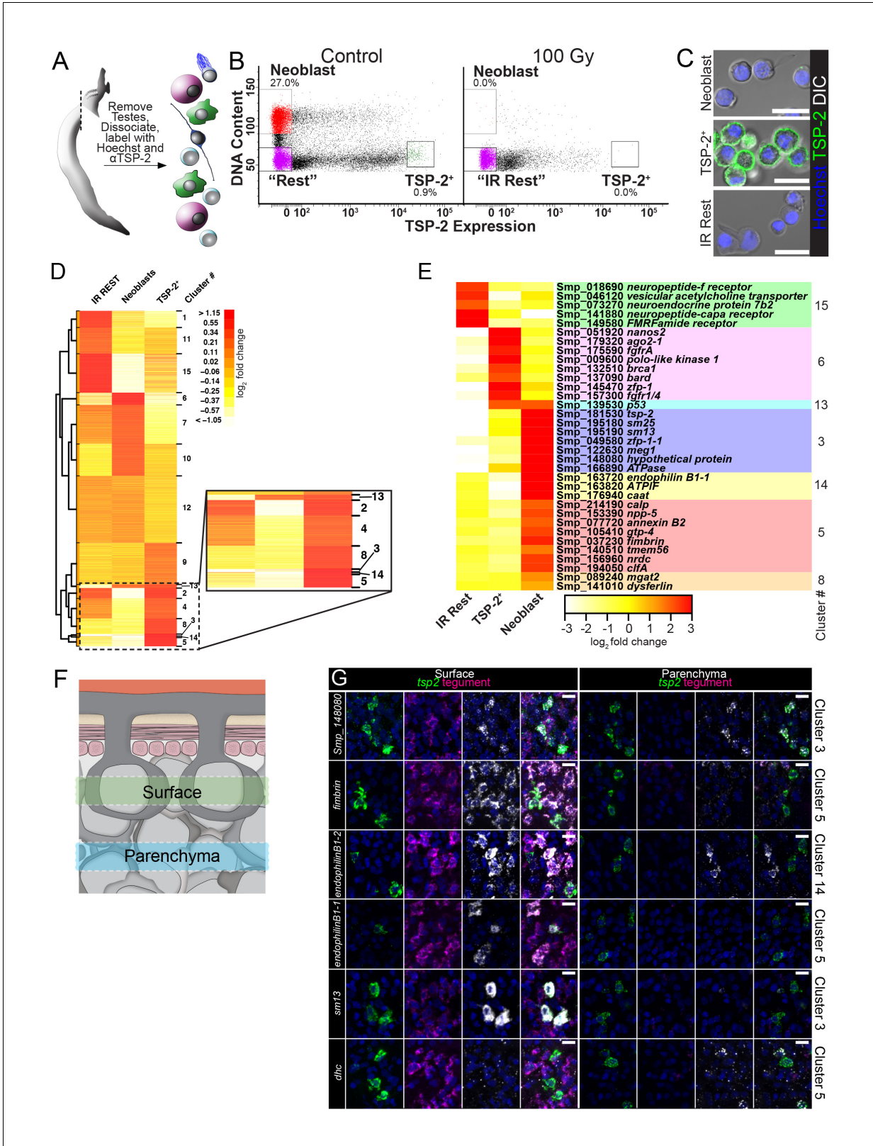
Figure 2. FACS purification and transcriptional profiling identifies molecules expressed in neoblasts and cells associated with the tegumental lineage. (A) Cartoon depicting FACS purification strategy. (B) FACS plots showing various cell populations in control and following gamma-irradiation. Percentages represent fraction of the number of cells in the boxed region over the total number of live cells. (C) Confocal micrographs of the sorted cell populations labeled with Hoechst and an anti-TSP-2 antibody. (D) Heatmap showing clustering analysis of genes expressed in the indicated cell populations. Figure 2 continued on next page
