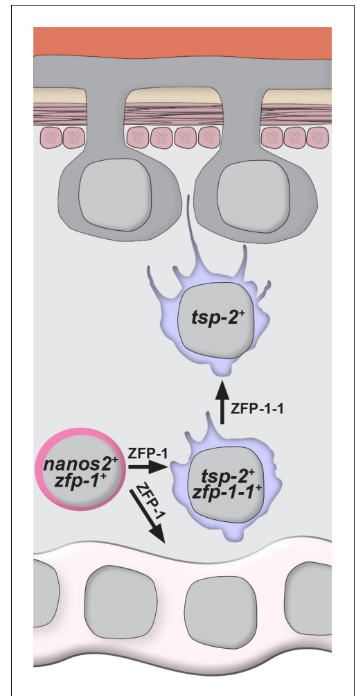
Figure 6. Model for the specification of new tegumental cells from neoblasts. Neoblasts (magenta cells) expressing nanos2 and zfp-1 specify large numbers of tsp-2 + cells. Some fraction of tsp-2 cells express zfp-1-1 . Within this tsp-2 compartment are cells that extend cytoplasmic projections ultimately fusing with the tegumental syncytium. Loss of zfp-1 function results in a general differentiation defect (i.e. loss of both tegument progenitors and gut cells) whereas loss of zfp-1-1 function results in a specific loss of tsp-2 + cells responsible for replenishing the tegument. In both cases, depletion of tsp-2 + cells causes a reduction in the total number of tegumental cell bodies.
